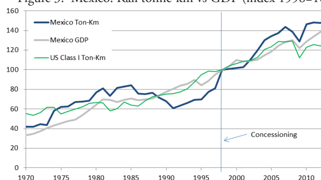
Figure 3. Mexico: Rail tonne-km vs GDP (index 1998=100)
